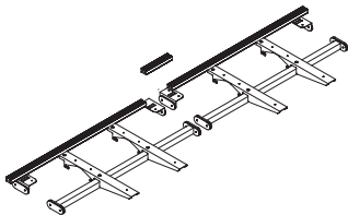
Support Structure
