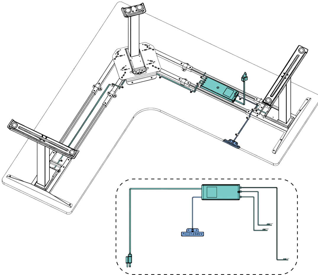
Parts View
