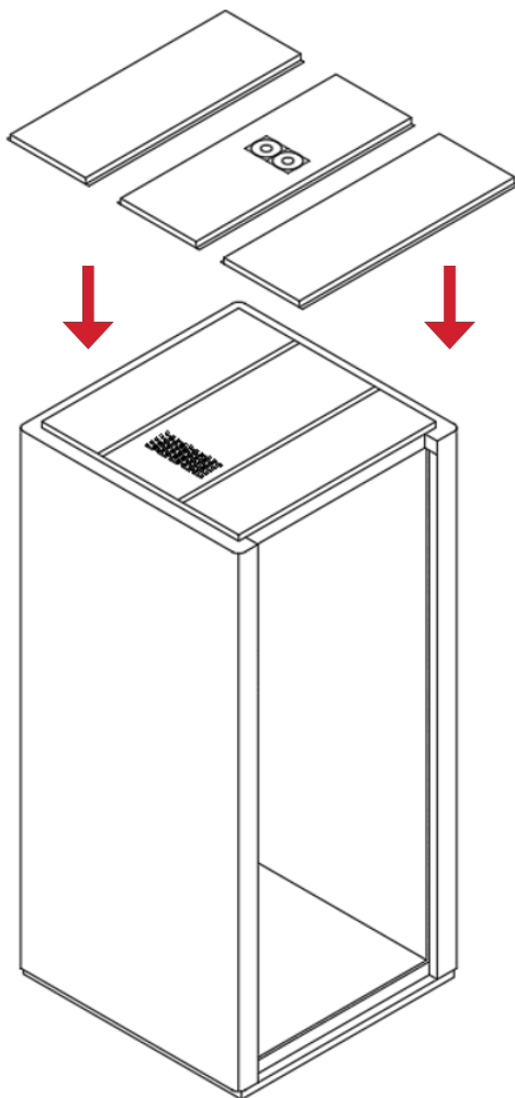
A. Place the ceiling covers on the ceiling frame
