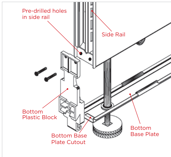
Bottom Plastic Block Assembly
